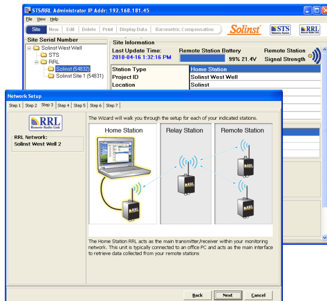
STS/RRL Gold Software Set-up Screens
